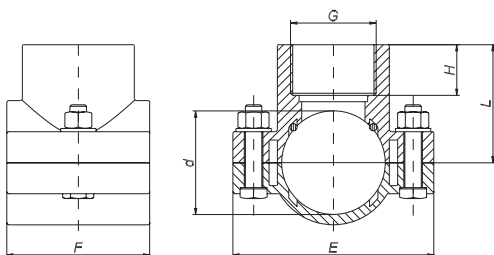
PRESA A STAFFA CLAMP SADDLE
